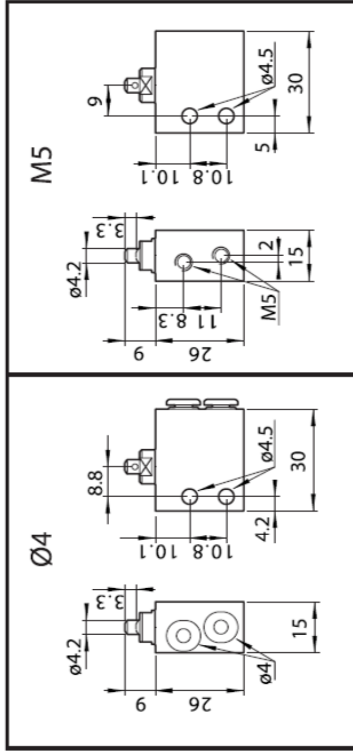
3/2-Wege Ventil NC / 3/2-way valve, NC
