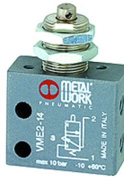
3/2-Wege Ventil NO 3/2-Way valve N.O.
