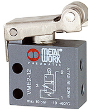
3/2-Wege Ventil NO 3/2-Way valve N.O.
